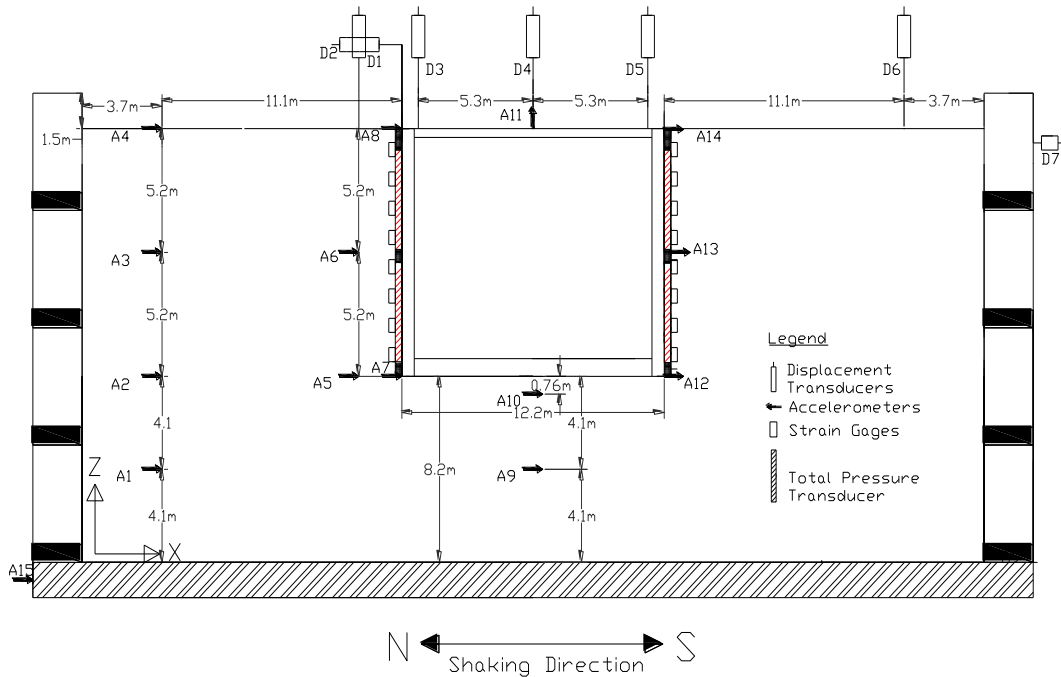
FIG. 2. Instrumentation layout for Test-1A (dimensions shown in prototype scale for a spin acceleration of 60 \text{ g} ). N and S represent North and South.
