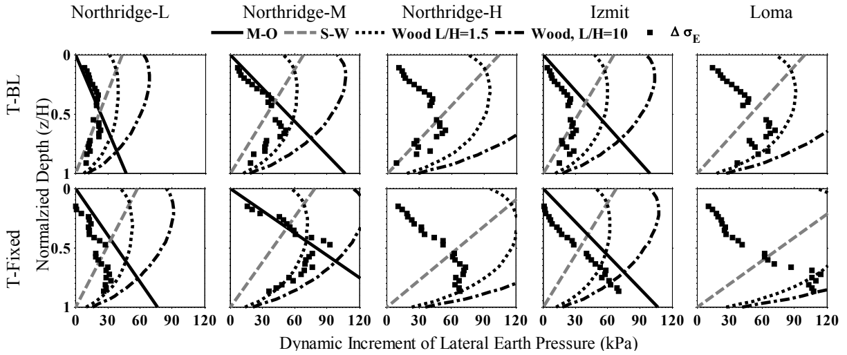
Figure 8. Dynamic lateral earth pressures at the time of maximum thrust in T-BL and T-Fixed.
