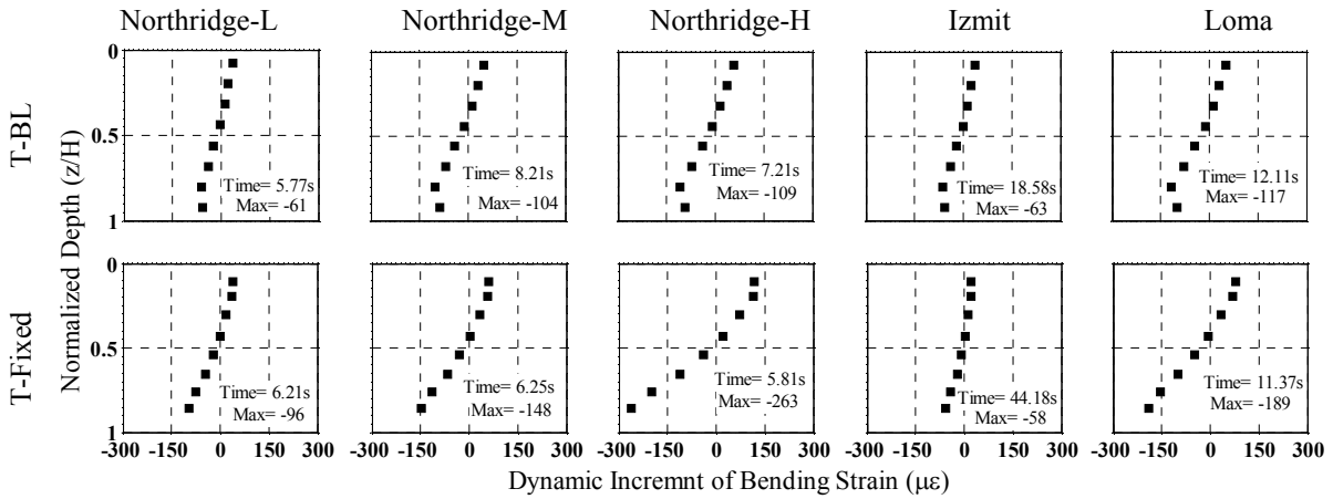
Figure 9. Dynamic increment of bending strains ( \Delta\epsilon_E ) at the time of maximum strain in T-BL and T-Fixed.
