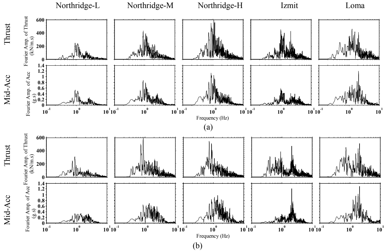
Figure 6. Fourier Amplitude Spectra of dynamic thrust and mid-depth structure acceleration in: (a) T-BL; (b) T-Fixed.
